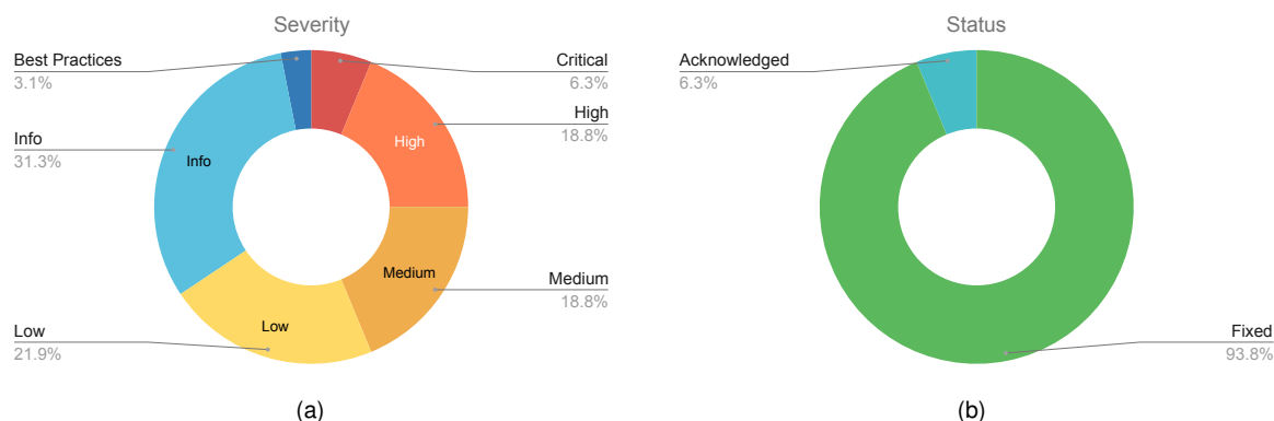
Fig. 1: Distribution of issues: Critical (2), High (6), Medium (6), Low (7), Undetermined (0), Informational (10), Best Practices (1). Distribution of status: Fixed (30), Acknowledged (2), Mitigated (0), Unresolved (0)
